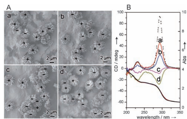
Figure 2. Reversal of the handedness of IHDSCs with increasing TMAPS/DNA molar ratio at 0^\circ\text{C} . A) SEM images and B) DRCD and UV/Vis spectra of the IHDSCs synthesized with TMAPS/DNA molar ratios of 3.5 (dotted line, also shown in Figure 1Bb), a) 4.5, b) 5.5, c) 6.5, and d) 7.5. The left- and right-handed impeller are denoted by + and –, respectively. The synthesis molar composition of DNA/ \text{MgCl}_2 /TMAPS/TEOS/ \text{H}_2\text{O} is 1:1: x :15:18 000. The pH value of synthesis solutions was 5.20.
