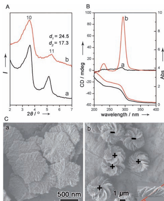
Figure 1. Structures and morphologies of the DSCs. A) XRD patterns, B) DRCD and UV/Vis spectra, and C) SEM images of the DSCs synthesized a) without and b) with addition of \text{Mg}^{2+} ions at 0^\circ\text{C} . Inset of SEM image (Cb): SEM image taken from the direction perpendicular to the impeller axis. Left- and right-handed impellers are denoted by + and –, respectively. The synthesis molar composition of DNA/ \text{MgCl}_2 /TMAPS/TEOS/ \text{H}_2\text{O} is 1: x :3.5:15:18 000, where x=0 (a) and 1 (b). The pH value of both synthesis solutions was 5.20.
